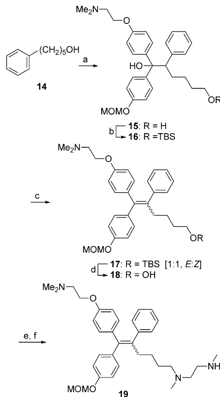
Scheme 2. (a) (i) t -BuOK (1 equiv), pentane, rt, 5 min, (ii) s -BuLi (2 equiv), TMEDA (2 equiv), 0 °C–rt, 1 h, (iii) 13 (0.17 equiv), THF, 0 °C–rt, 4 h, 80%; (b) TBS-Cl, imidazole, DMAP (cat.), CH 2 Cl 2 , rt, 12 h, 79%; (c) SOCl 2 , pyridine, –10 °C, 4.5 h, 99%; (d) TBAF, THF, rt, 6 h, 98%; (e) CBr 4 (1.2 equiv), PPh 3 (1.2 equiv), CH 2 Cl 2 , 0 °C–rt, 1 h; (f) MeNHCH 2 CH 2 NHMe (10 equiv), CH 3 CN, rt, 12 h, 73% two steps.
