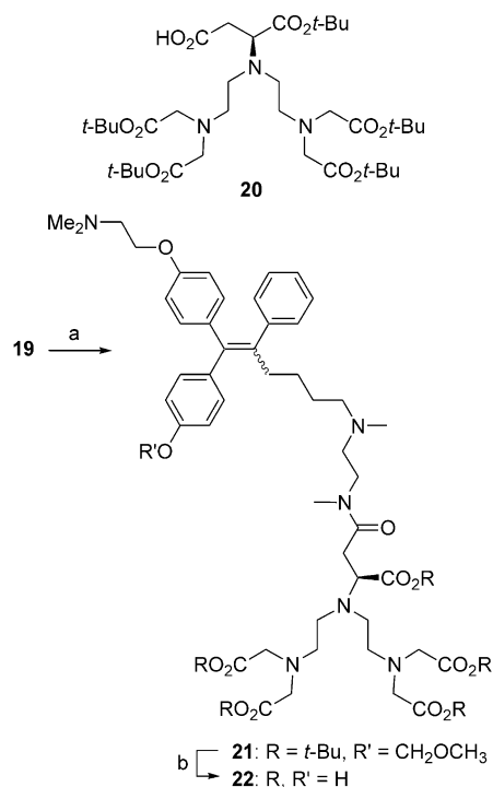
Scheme 3. (a) DCC, HOBT, 20 , \text{CHCl}_3 , 64%; (b) TFA, Anisole (30 equiv), \text{CH}_2\text{Cl}_2 , -10^\circ\text{C} – rt, 12 h.
