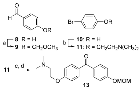
Scheme 1. (a) NaH (1.1 equiv), MOMCl (1 equiv), DMF, 0 °C–rt, 4.5 h, 74%; (b) K 2 CO 3 (4 equiv), Me 2 NCH 2 CH 2 Cl·HCl (2 equiv), DMF, rt, 24 h, 80%; (c) (i) Mg, THF, reflux 2 h, (ii) 9 , THF, 0 °C–rt, 3.5 h, 97%; (d) MnO 2 (20 equiv), pentane, rt, 18 h, 98%.
