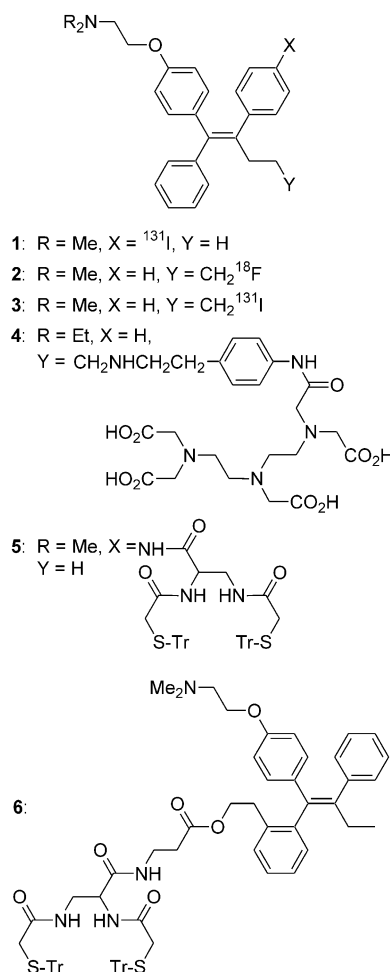
Figure 2. Tamoxifen radionuclides and chelates for imaging. Tr = \text{CPh}_3 .
