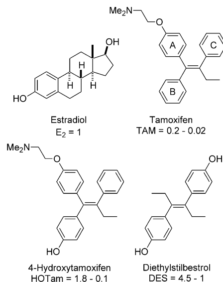
Figure 1. Structures and approximate relative binding values of common estrogen receptor ligands. 4,12,13
